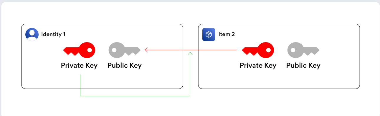
Fig. 3 Access grant (relation)
