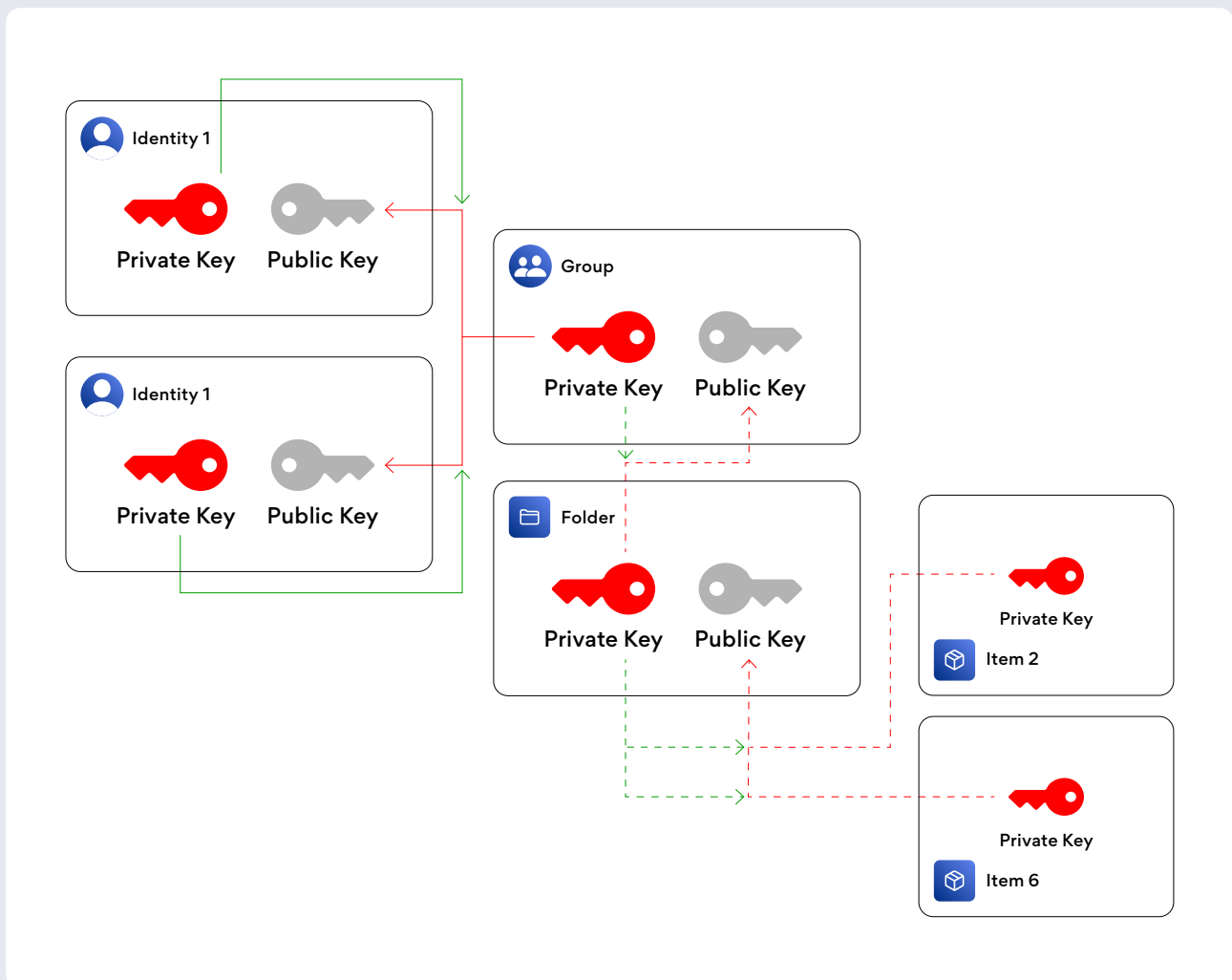
Fig. 6 Accessing items grouped in a folder via group
