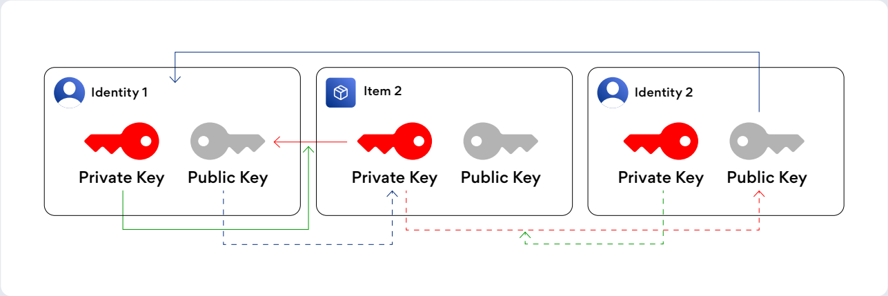
Fig. 4 Sharing an item with another identity
