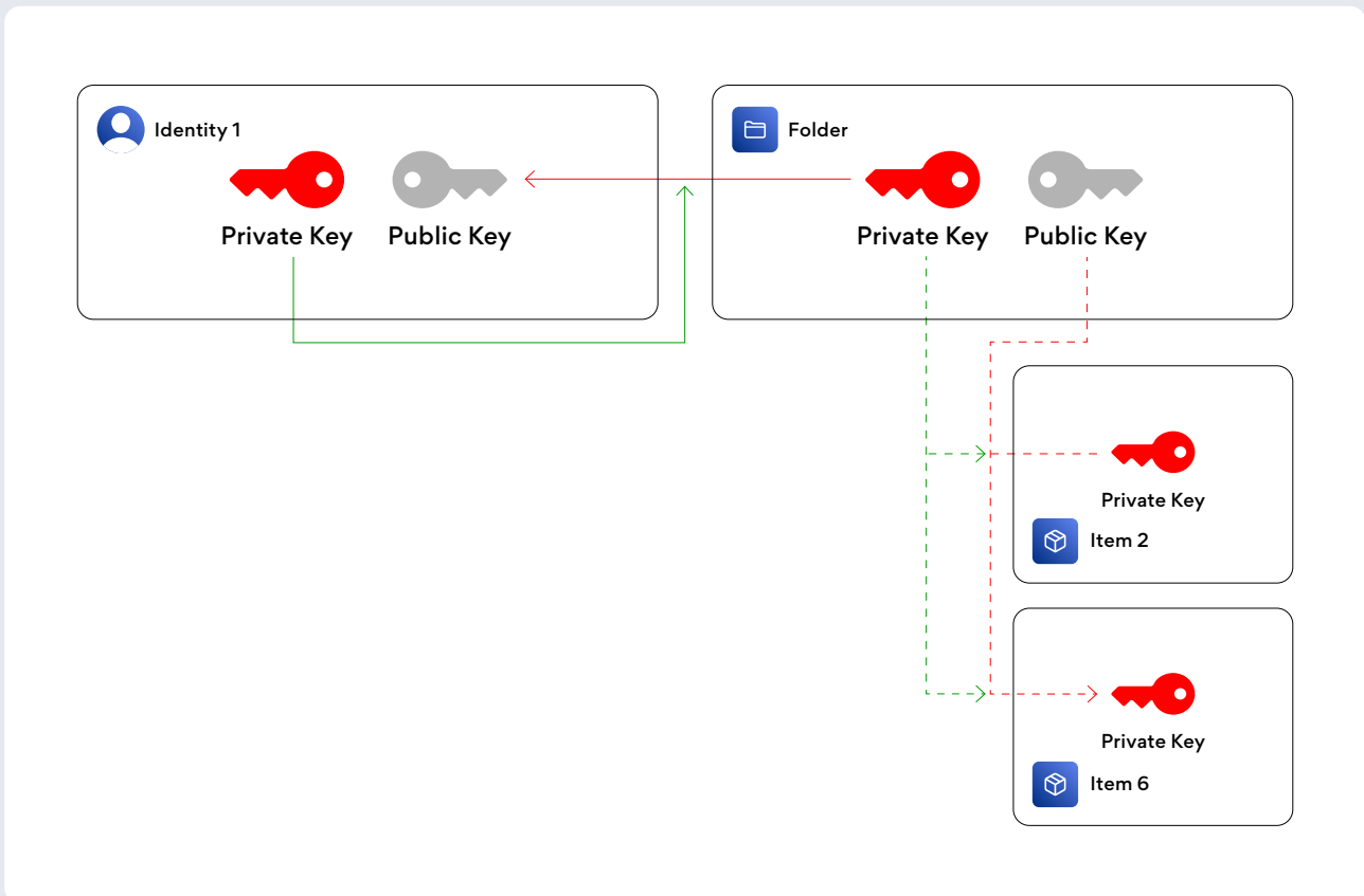
Fig. 5 Accessing items grouped in a folder
